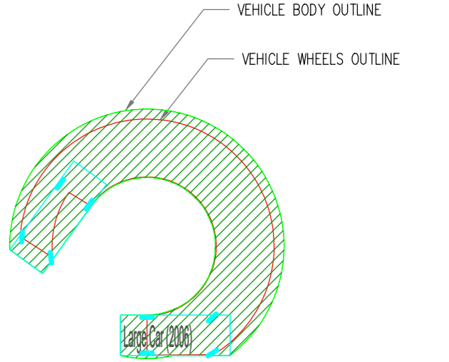
SWEPT PATH PLAN.
